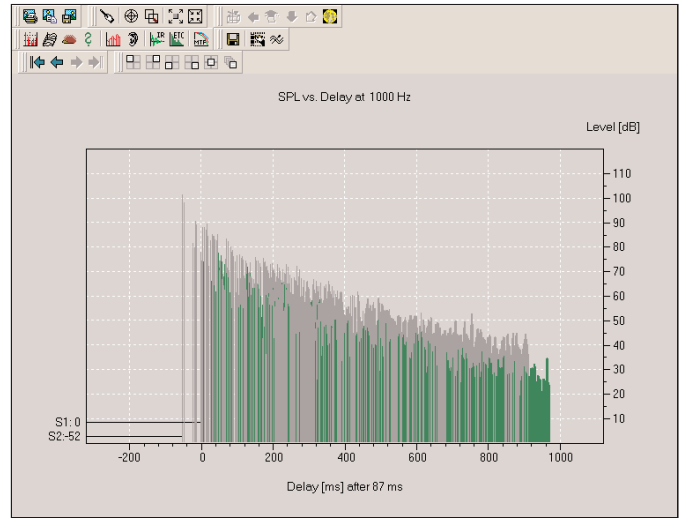
A typical AURA Reflectogram
