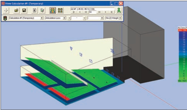
Typical ALCons Intelligibility Display
