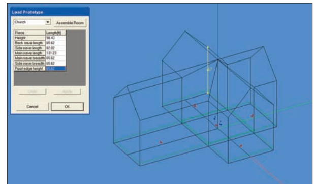
One of 33 prototype room models that speed room modeling
