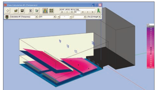
STI displayed on Audience Areas
