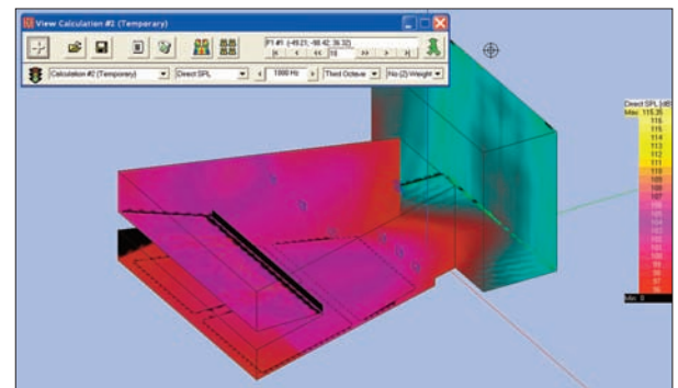
Direct SPL displayed on room surfaces
