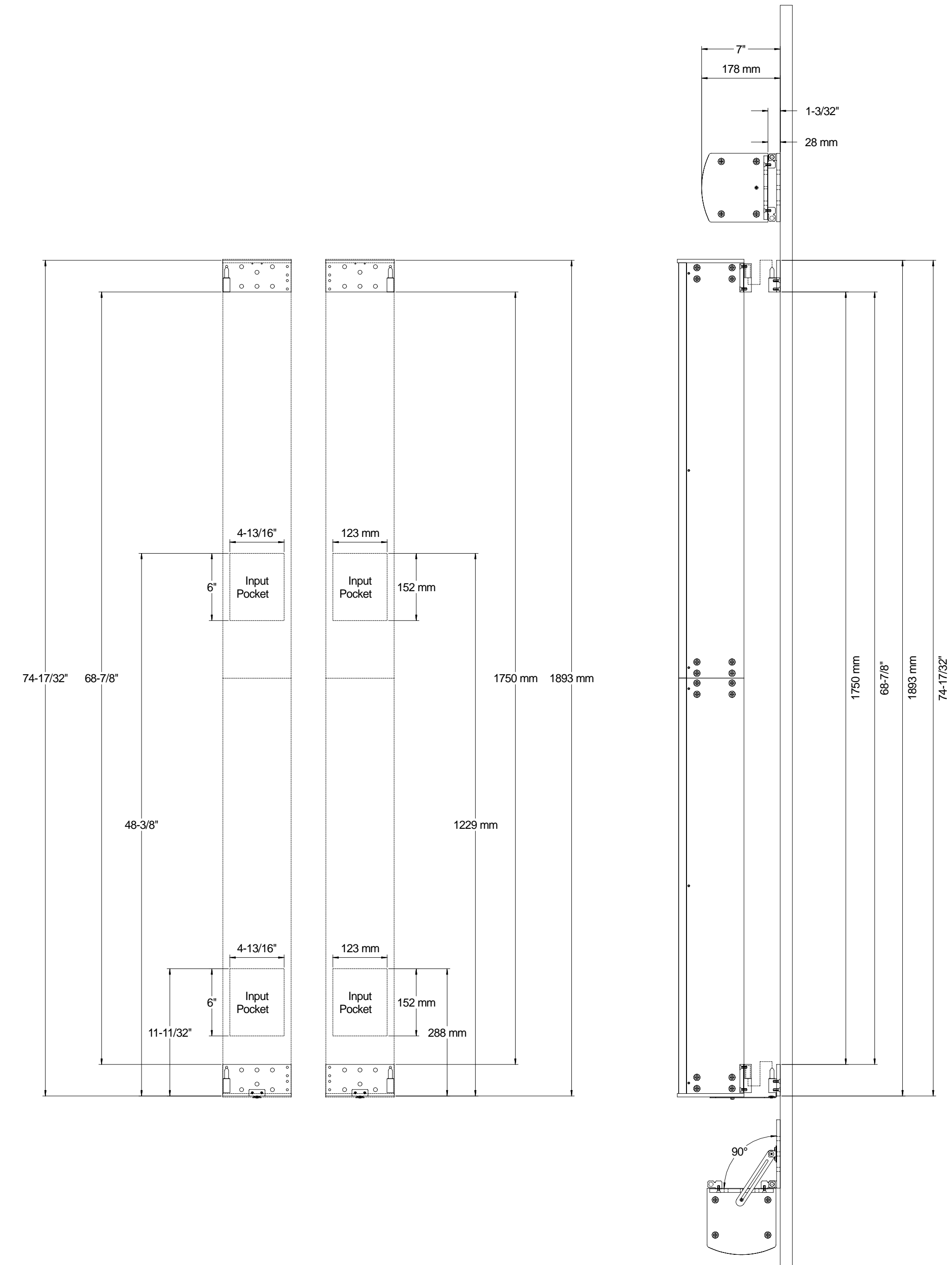
IC16R Install Dimensions
