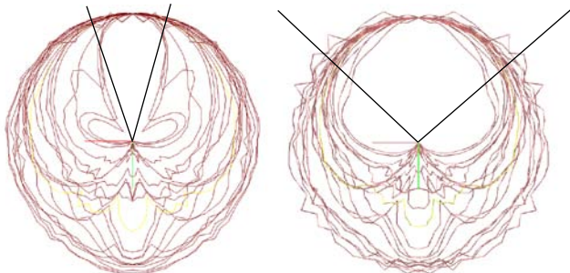
Conventional Transducer
