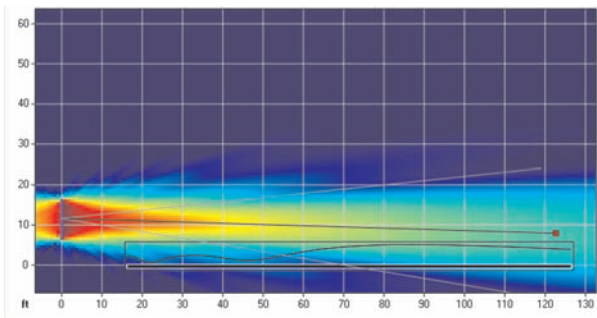
BeamWare display of an IC24A illustrating the reduced grating offered by ICONYX IC-A series arrays with their improved algorithms and dual HF tweeters.
