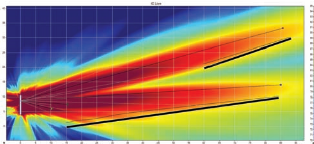
Beamware display of an Iconyx IC16 array's dual beam output..
