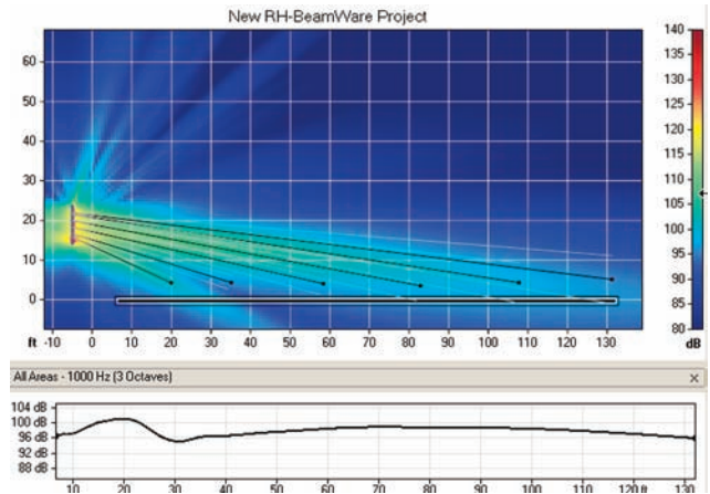
Beamware display showing the multi-beam and movable acoustic centers capabilities of the IC24A Iconyx array.
