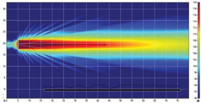
BeamWare display of an Iconyx array at 4 kHz illustrating the reduced grating offered by Iconyx IC-R-II series arrays with their improved algorithms and evenly spaced triple dome HF tweeters.
