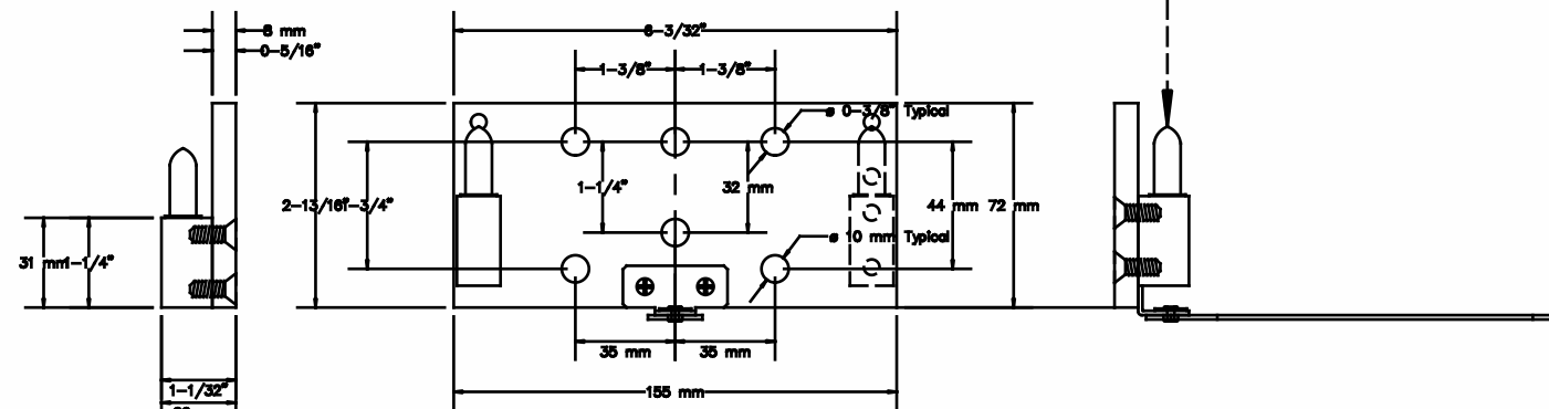
Wall Bracket
